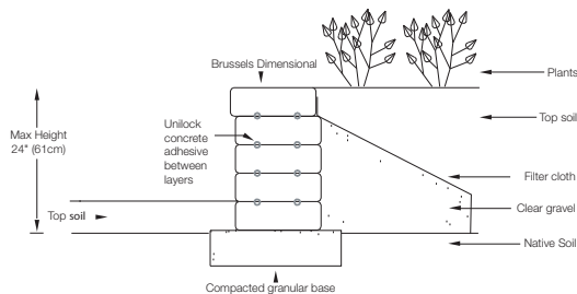
GRAVITY WALL SECTION
